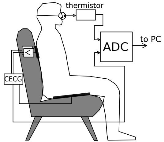
Fig. 1. Experiment setup
