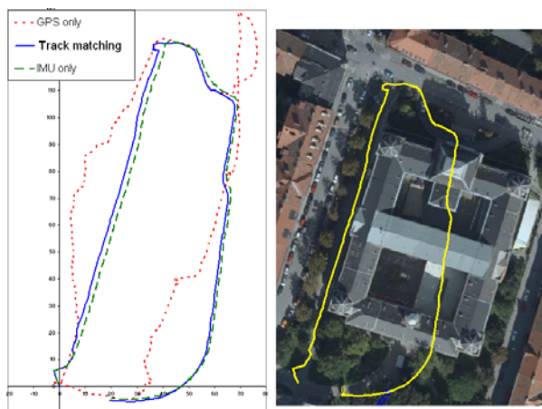
Figure 2 Different sensor-fusion methods with best results for track matching algorithm (<2m indoor and outdoor for 900m)
