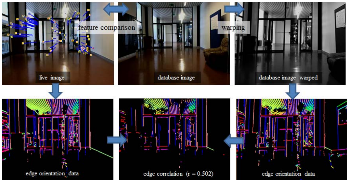
Figure 3 Common features in the live image (top left) and the database image (top center) are used to warp the database image on the live image frame (top right). Then the respective edge orientations (represented by the pseudo colors) are extracted (bottom left and right) and their correlation is determined (bottom centre)
